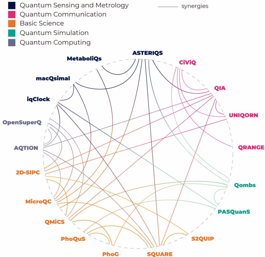
Figure 2: Visual summarisation of the synergies among Quantum Flagship projects
